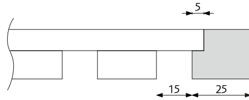
Cut felt with end strip
