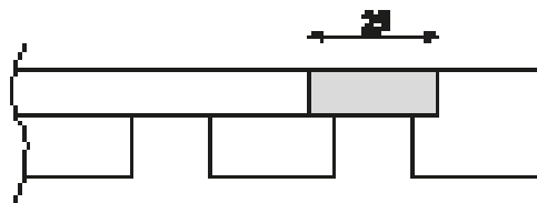
End strip with splicing strip
